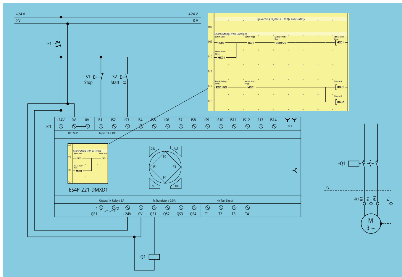
Figure 29: Self-switching with easySafety prevents automatic restart with voltage recovery
