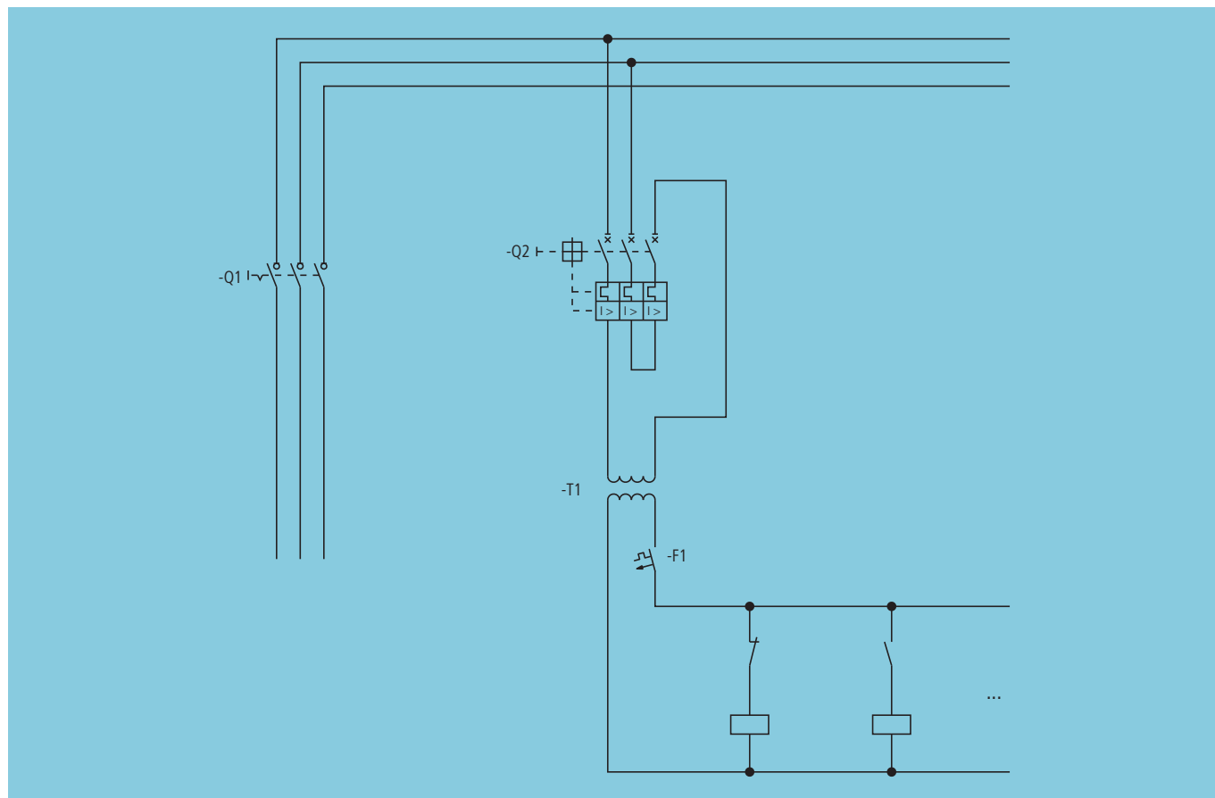
Figure 36: PELV extra low voltage with safe isolation
