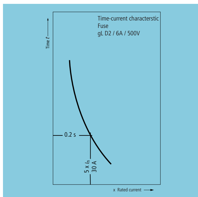
Figure 40: Example: Time-current characteristic of a 6 A fuse
