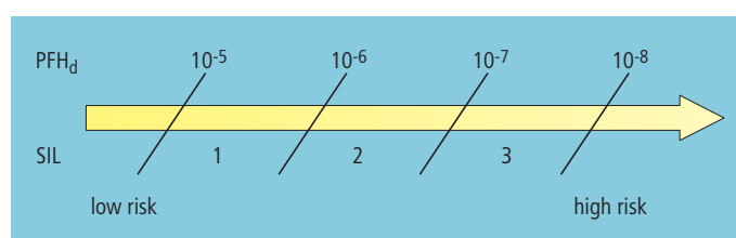
Figure 51: Average probability of failure
