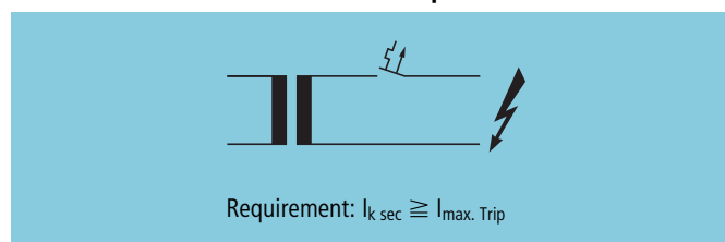
Figure 39: Determination of short-circuit devices
