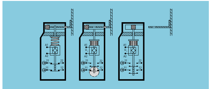
Figure 59: Spring force locking device
