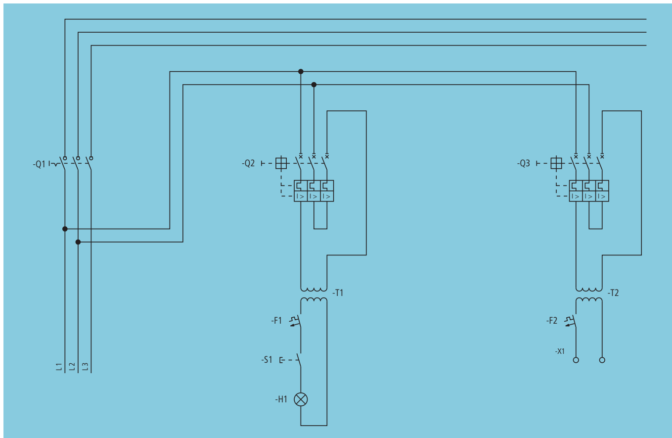
Figure 35: Protective isolation
