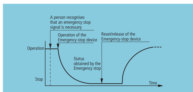
Figure 61: Function sequence emergency stop
