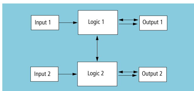
Figure 76: Structure for category 4
