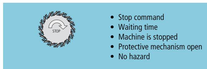
Figure 55: Interlock equipment with guard locking for increased personnel protection
