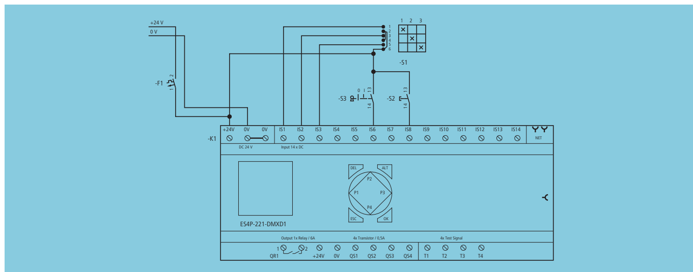
Figure 24: Safe operating mode selection with easySafety
